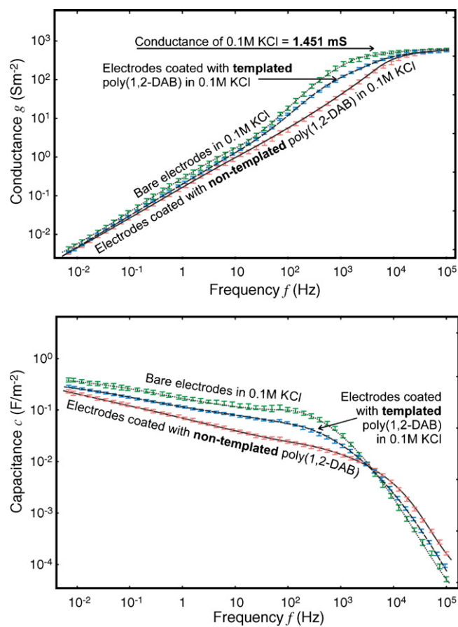
Fig. 5. Conductance and capacitance as a function of frequency for a pair of 0.79 mm 2 gold disk electrodes either uncoated or coated with C 16 EO 8 templated or non-templated poly(1,2-DAB) as indicated in the graph. Electrodes were immersed in 0.1 M KCl.
