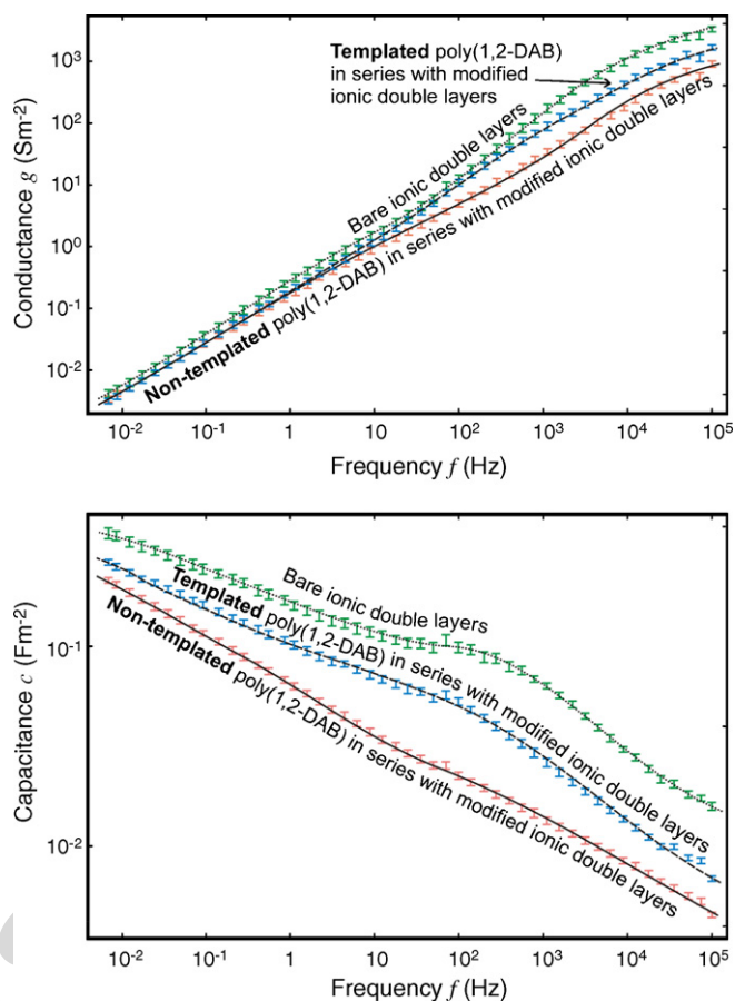
Fig. 6. Conductance and capacitance of the uncoated gold electrodes and the C 16 EO 8 templated and non-templated poly(1,2-DAB) films, respectively, after subtraction of the contribution of the conductance of the electrolyte in series with the electrodes. This allows the differences between the templated and non-templated films to be more readily discerned. The dispersion of the conductance and capacitance for the uncoated electrode now refers to the ionic double layer formed at the electrode–solution interface.
