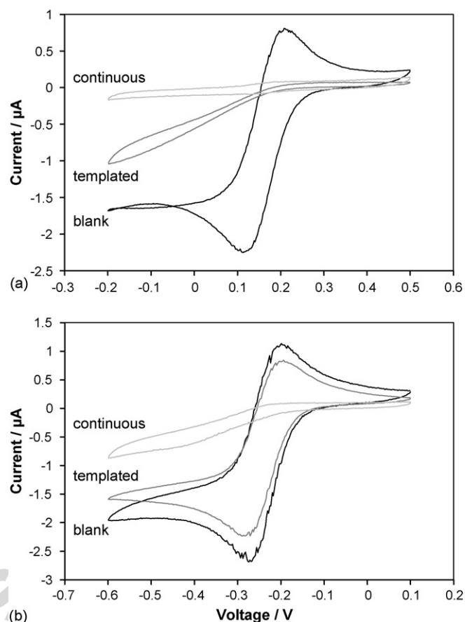
Fig. 2. CVs of various 0.79 mm 2 gold disk electrodes in 5 mM ferricyanide (a) and 5 mM ruthenium hexaammine (b). Electrodes are labelled “continuous” (non-templated poly(1,2-DAB) film), “templated” (Brij 56 templated poly(1,2-DAB) film), and “blank” (blank gold disk electrode). Scan rate, 5 mV/s.
